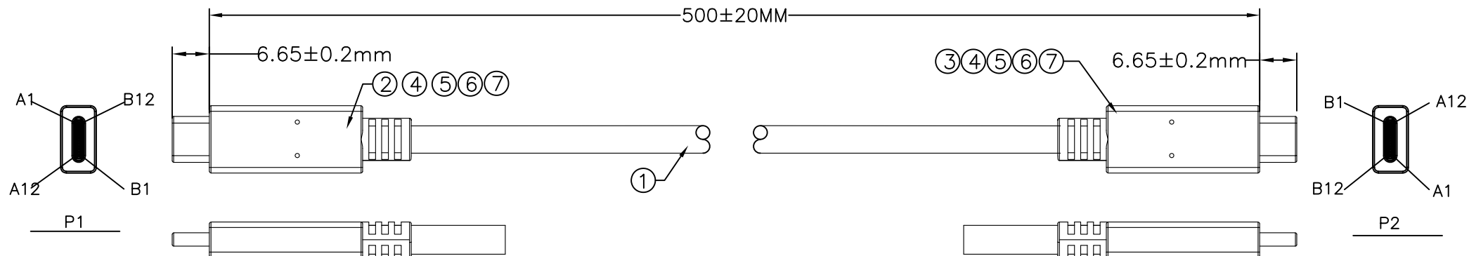
Pin Assignment
