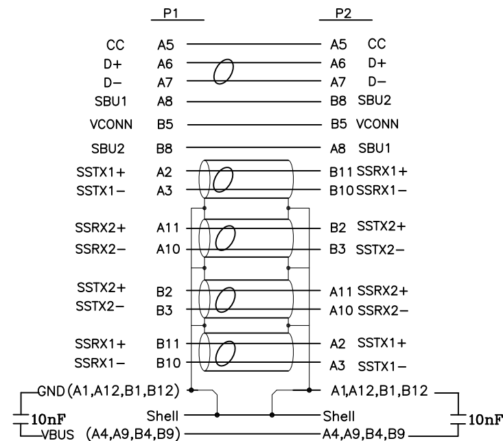
Pin Assignment
