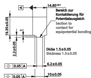
Dimensions E-DAT modul Cut-out
